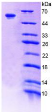
Figure. SDS-PAGE
