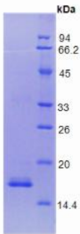
Figure. SDS-PAGE
