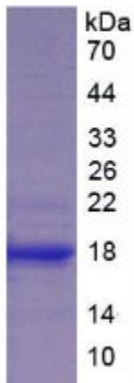
Figure. SDS-PAGE
