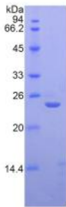
Figure. SDS-PAGE
