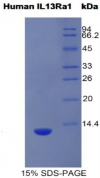
SDS-PAGE Image
