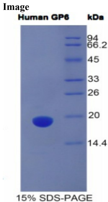
SDS-PAGE Image
