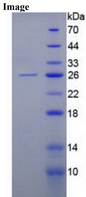
Figure. SDS-PAGE
