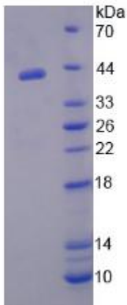
SDS-PAGE Image
