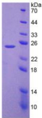
Figure. SDS-PAGE
