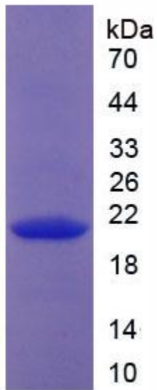
SDS-PAGE Image
