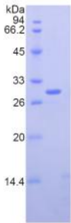
Figure. SDS-PAGE
