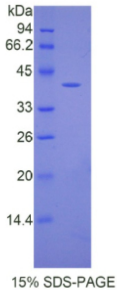
SDS-PAGE Image
