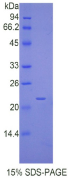
SDS-PAGE Image
