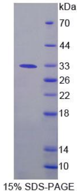
Figure. SDS-PAGE
