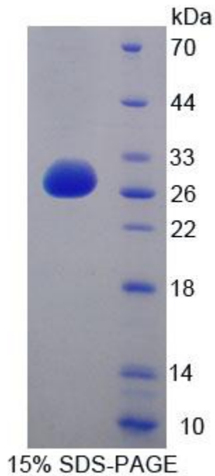
Figure. SDS-PAGE
