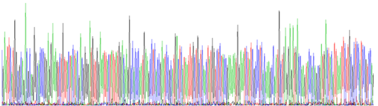
Figure. SDS-PAGE
