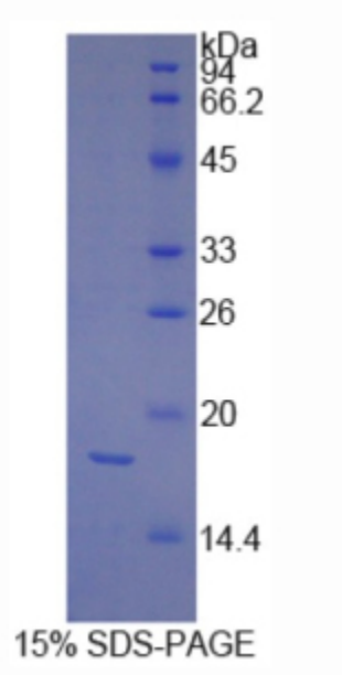
SDS-PAGE Image
