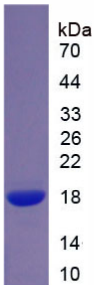
Figure. SDS-PAGE
