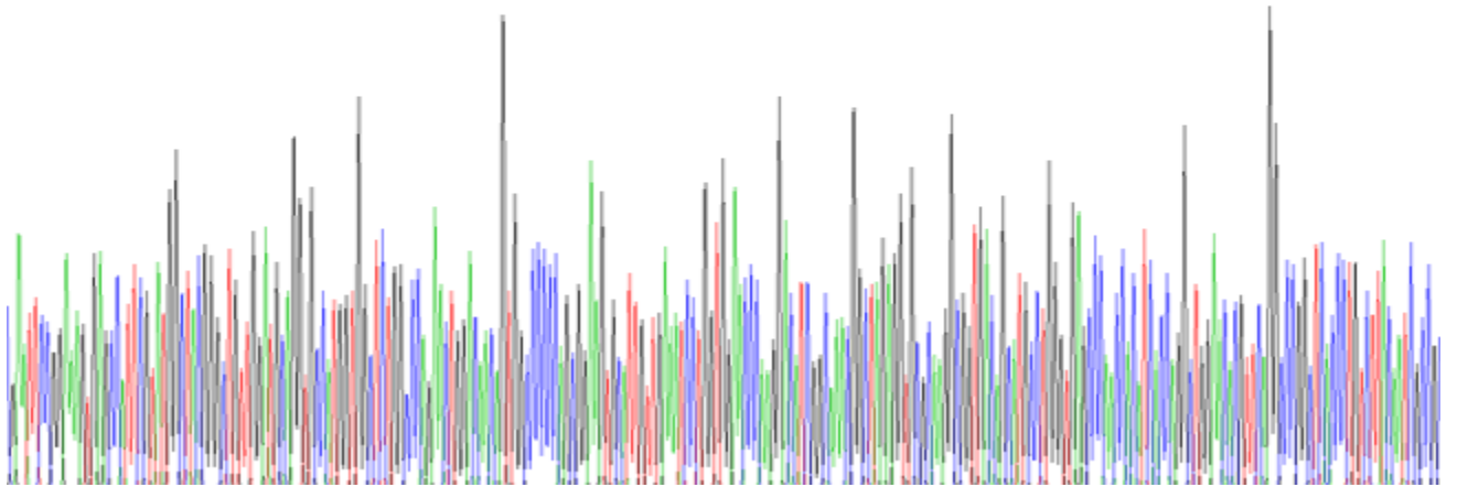
Figure. SDS-PAGE
