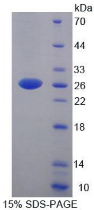
SDS-PAGE Image
