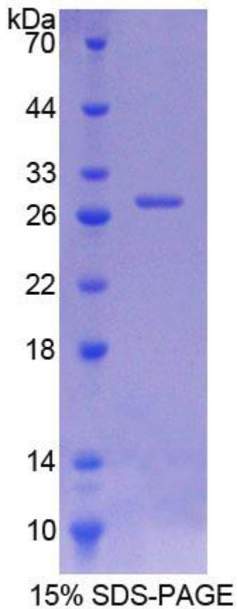
SDS-PAGE Image
