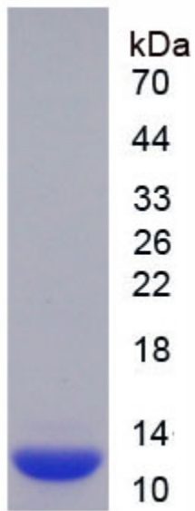
Figure. SDS-PAGE
