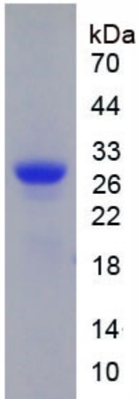
Figure. SDS-PAGE
