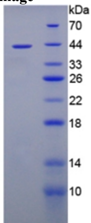
SDS-PAGE Image
