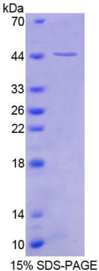
SDS-PAGE Image
