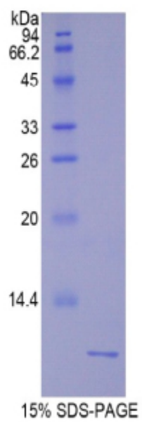
SDS-PAGE Image
