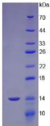
Figure. SDS-PAGE
