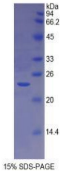
SDS-PAGE Image
