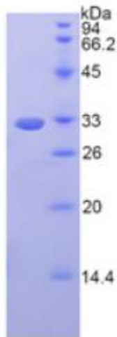
SDS-PAGE Image
