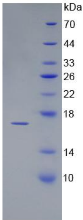
15% SDS-PAGE SDS-PAGE Image
