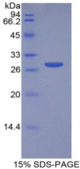
SDS-PAGE Image
