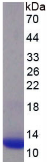
Figure. SDS-PAGE
