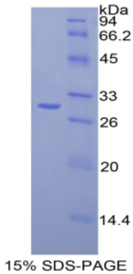
SDS-PAGE Image
