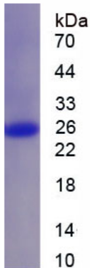
Figure. SDS-PAGE
