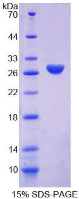
SDS-PAGE Image
