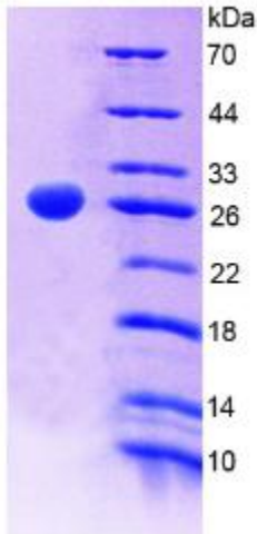
SDS-PAGE Image
