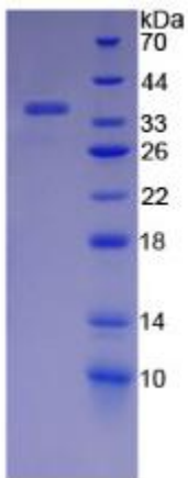
Figure. SDS-PAGE
