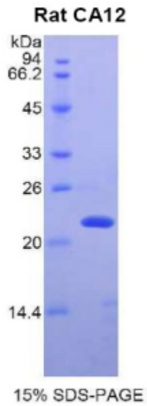
SDS-PAGE Image
