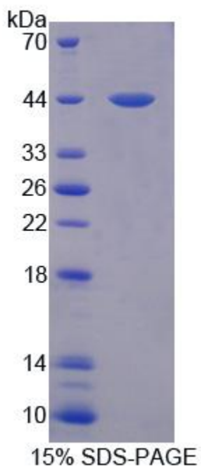
SDS-PAGE Image
