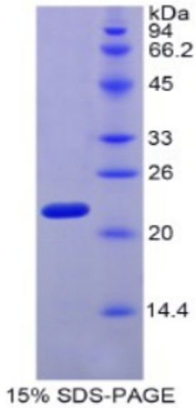
SDS-PAGE Image
