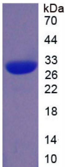
Figure. SDS-PAGE
