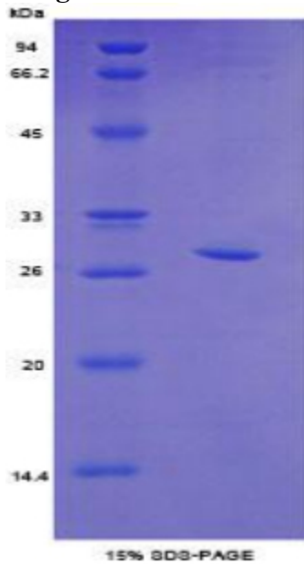
SDS-PAGE Image
