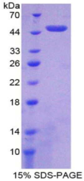
SDS-PAGE Image
