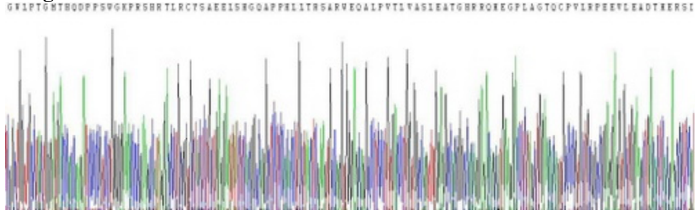
Figure. SDS-PAGE
