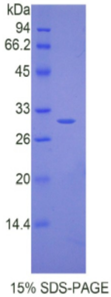
SDS-PAGE Image
