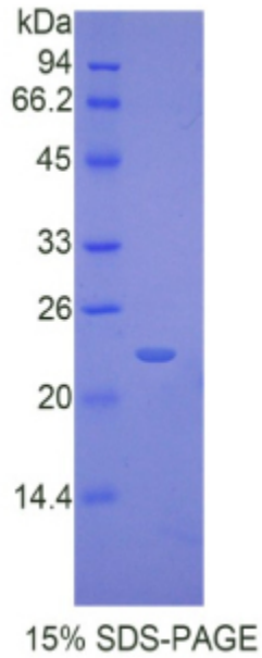
SDS-PAGE Image
