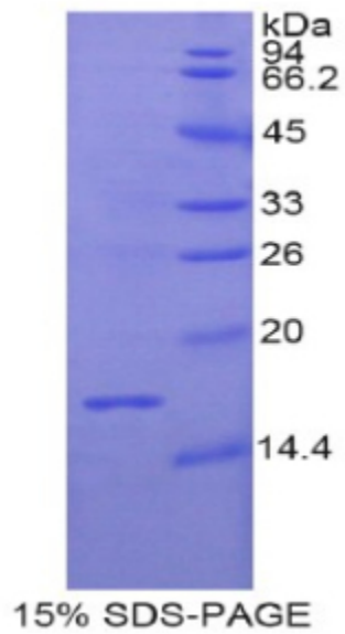
SDS-PAGE Image
