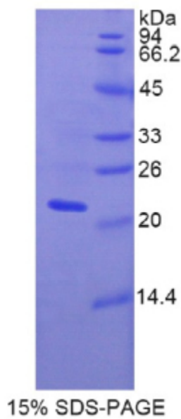
SDS-PAGE Image
