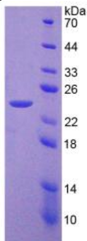
SDS-PAGE Image
