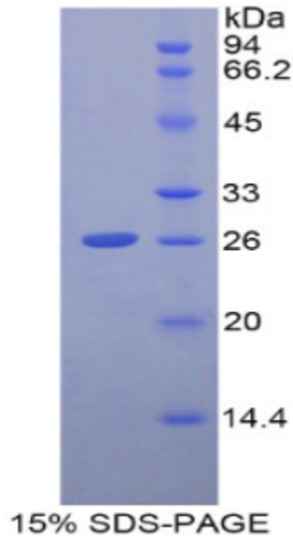
Figure. SDS-PAGE
